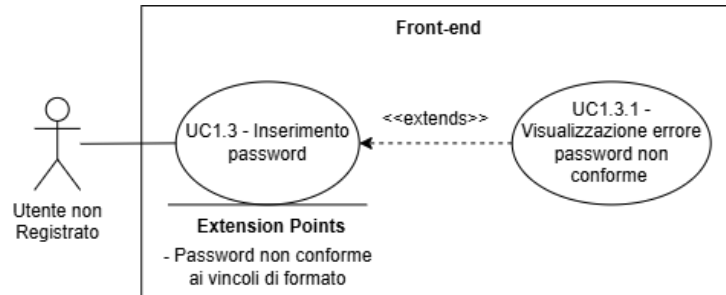
Figure 4: UC1.3 - Inserimento password
