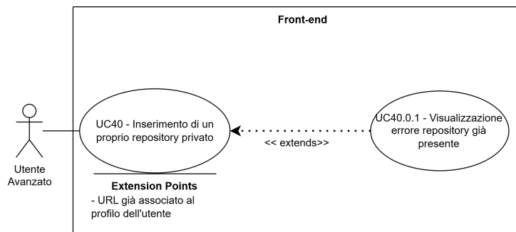
Figure 55: UC40 - Inserimento repository privato
