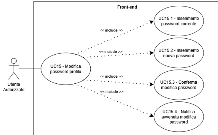
Figure 26: UC15 - Modifica password
