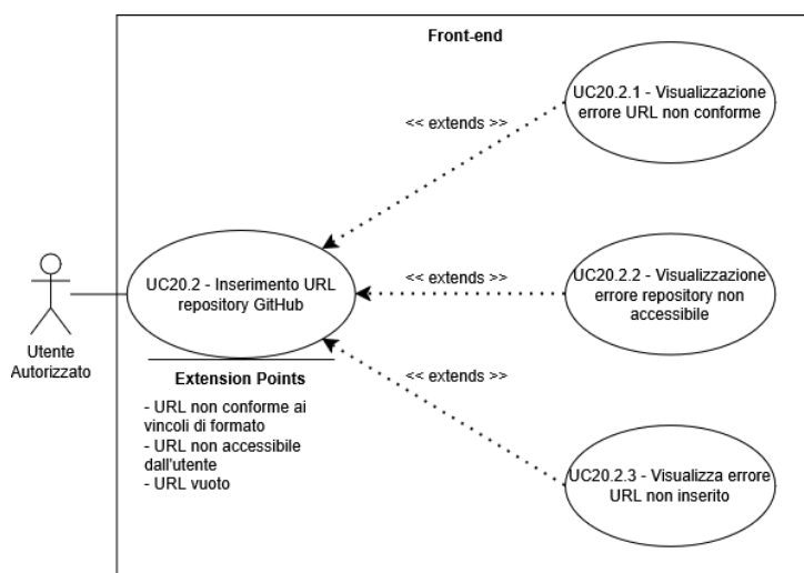
Figure 36: UC20.2 - Inserimento URL repository GitHub
