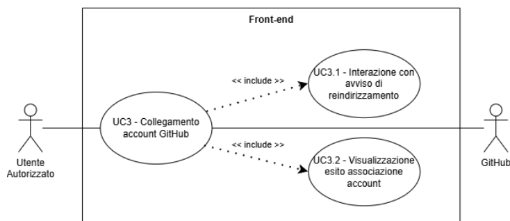
Figure 6: UC3 - Collegamento account GitHub
